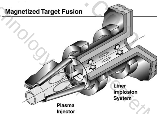
Fig. 1. MTF schematic showing plasma formation region and liner implosion section.
