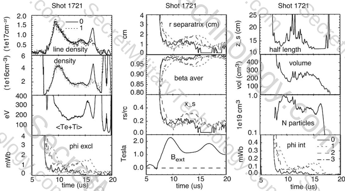
Fig. 5. Analysis of one shot showing many quantities that can be inferred from excluded flux and interferometer (0—on axis; 1–2 cm—off axis) data. For the internal flux plot (phi int) indexes 1, 2 represent flux loops that straddle the midplane axially and 0, 3 loops are closer to the ends of the theta coil.
