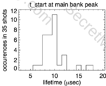
Fig. 7. Histogram summarizing 35 shots and the typical FRC lifetimes. For these shots, we varied fill pressure from 30 to 60 mtorr, as well as the trigger timing for PI and crowbar relative to the main bank trigger.
